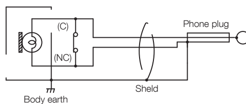
Circuit diagram
