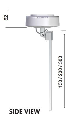
CEILING MOUNTING
