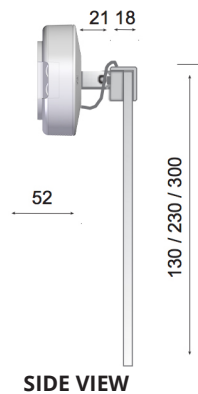
WALL MOUNTING
